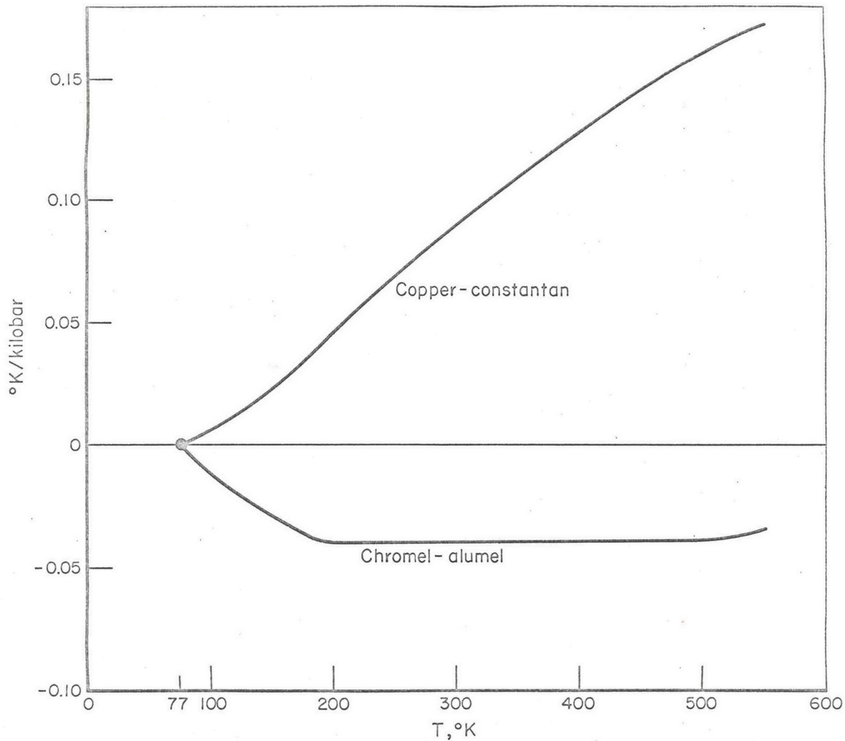
TEMPERATURE CORRECTION FOR PRESSURIZED THERMOCOUPLES Lead out at 78^{\circ}\text{K} ; hot junction at T
